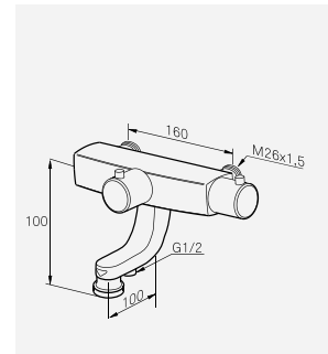
Badkarsblandare MA 15 08 00 RSK-nr 834 39 58
